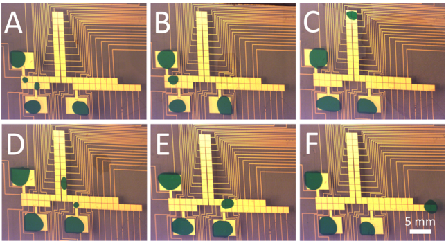
Figure 3. Image sequence of on-chip DMF transformation. (A) Images of filled reservoirs and generation of droplets containing DH5α cells or GFP plasmid, followed by (B) mixing of droplets at 4 °C. (C) Droplet transferred to 42 °C region of device and then (D) moved to 4 °C device region during generation of droplet consisting of LB and AMP. (E) Droplets are then merged and allowed to recover at 4 °C, then (F) transferred to a 37 °C culture chamber.
